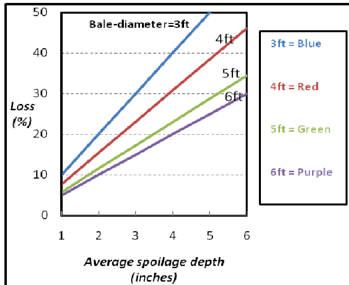
Figure II Depth of Spoilage and Bale diameter (Buckmaster, 1993)
